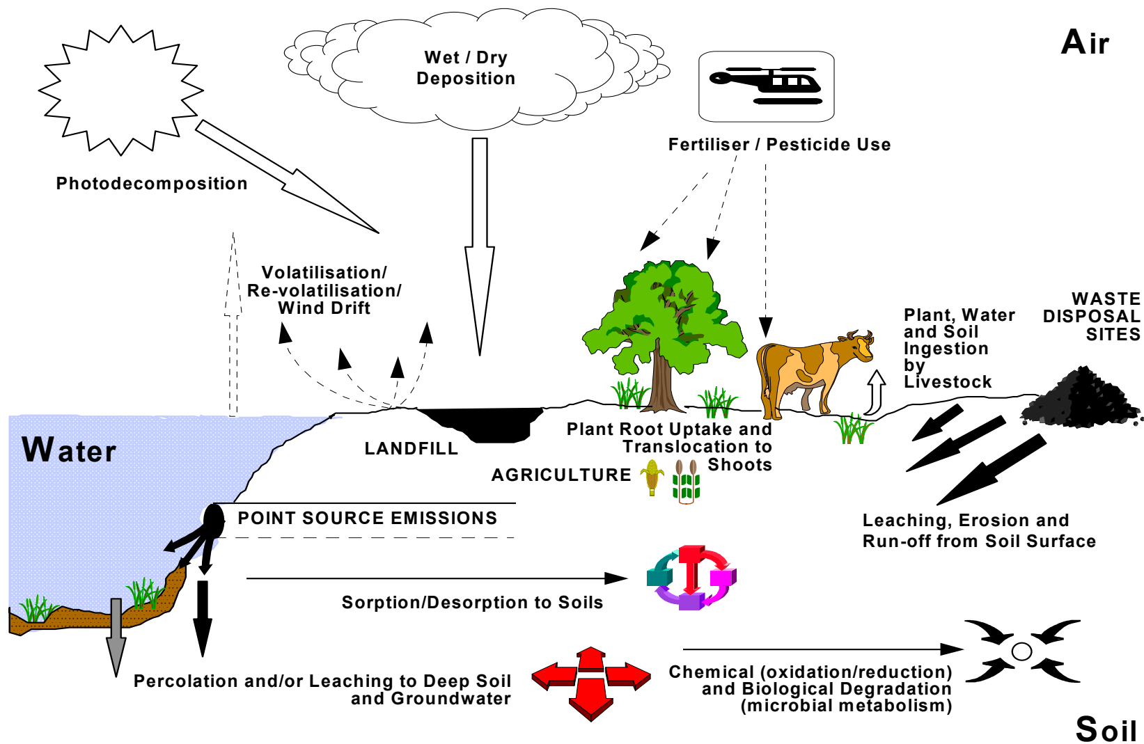
Figure 3.4 Main mechanisms of chemical cross-transfer between soil/sediment and other environmental compartments
