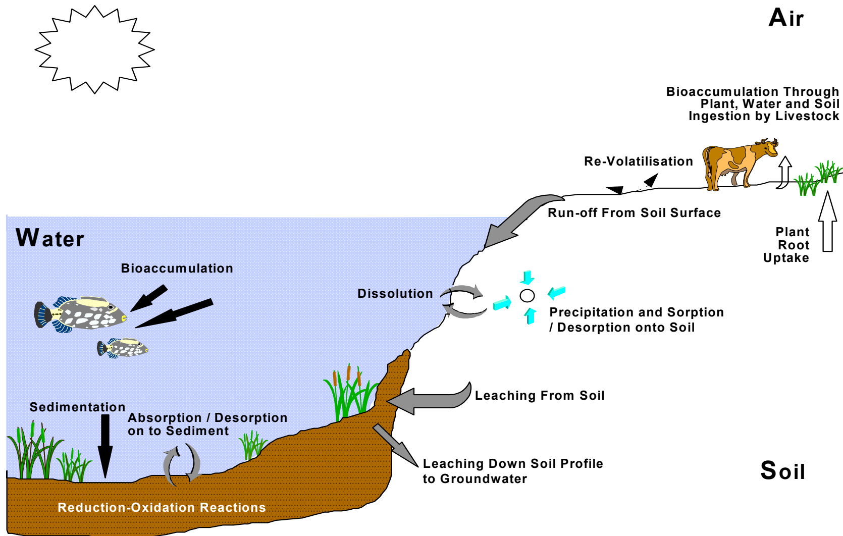
Figure 3.6 Main pathways of chemical transfer between environmental compartments
