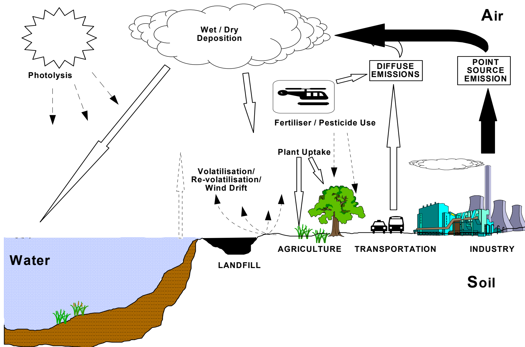
Figure 3.2 Main mechanisms of chemical cross-transfer between air and other environmental compartments
