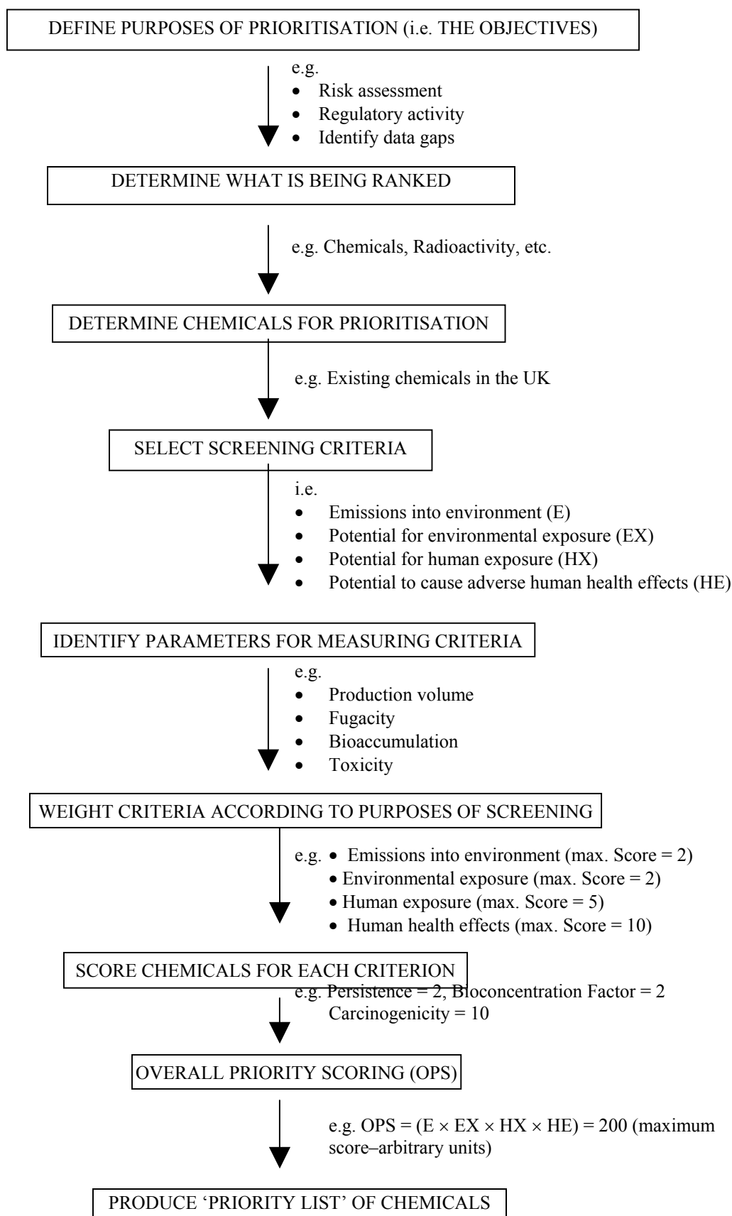
Figure 3.1 Conceptual model of a representative prioritisation scheme
