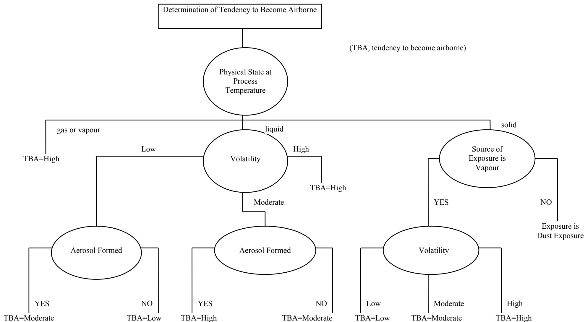
Figure 3.3 Determination of the tendency of a chemical to become airborne (from European Commission, 1996)
