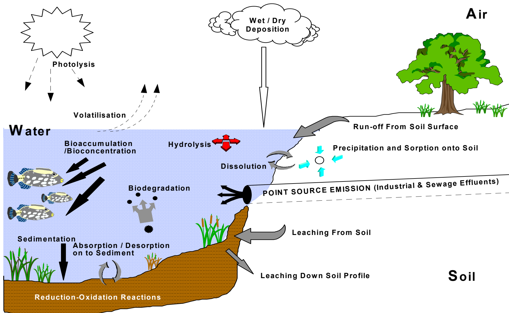
Figure 3.5 Main mechanisms of chemical transfer between water and other environmental compartments
