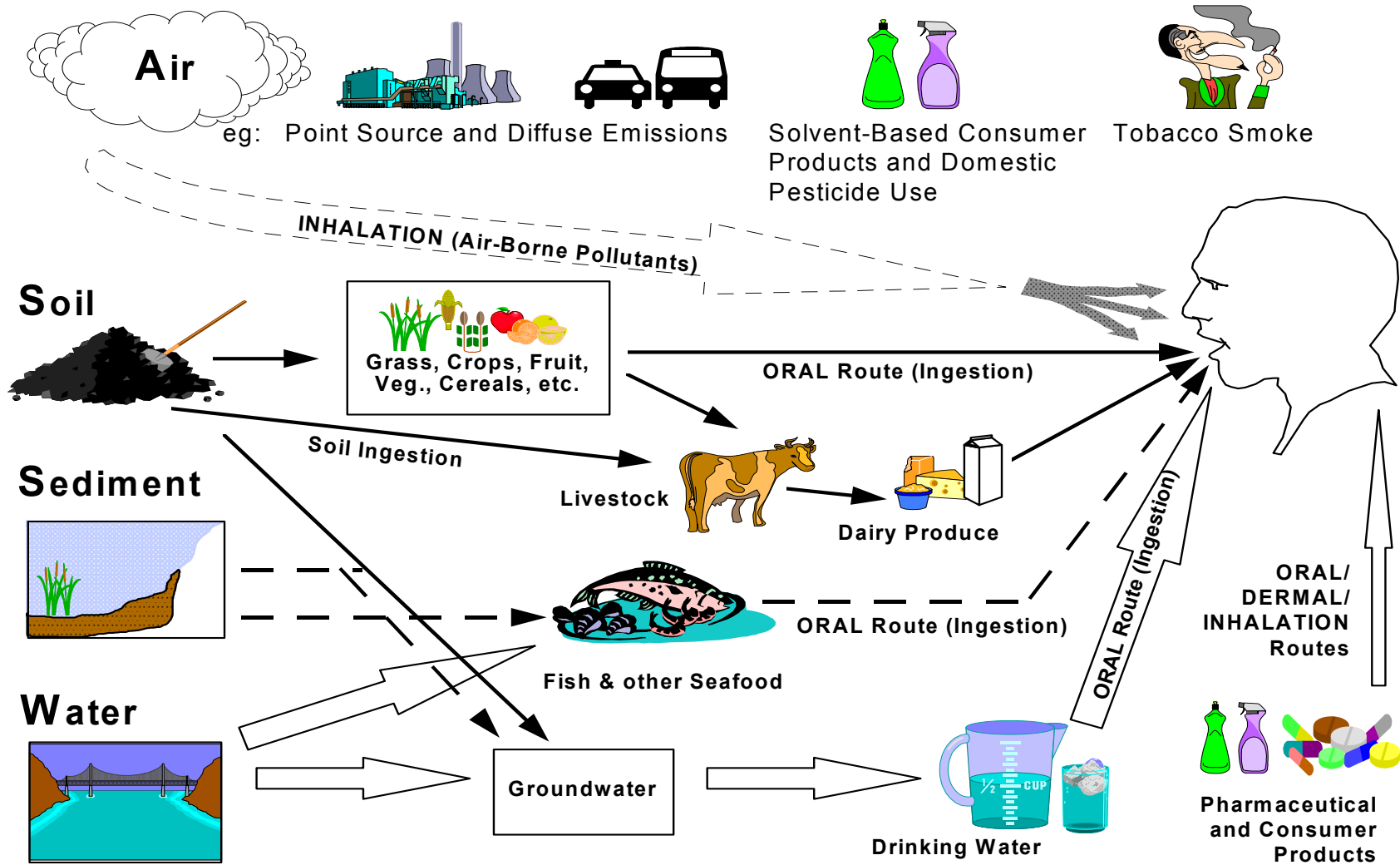
Figure 3.7 Main sources and routes of non-occupational chemical uptake by humans
